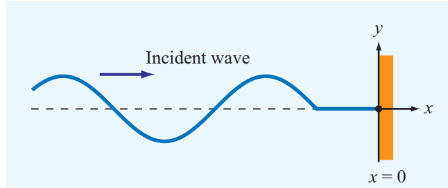
Figure P1.7 Wave on a string tied to a wall at x = 0 (Problem 1.7).
